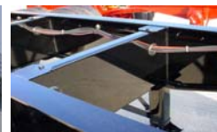
Full depth cross-members w/bolted gussets
